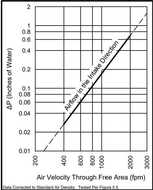
AIR PERFORMANCE
