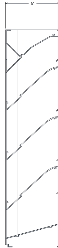
Vertical Section
