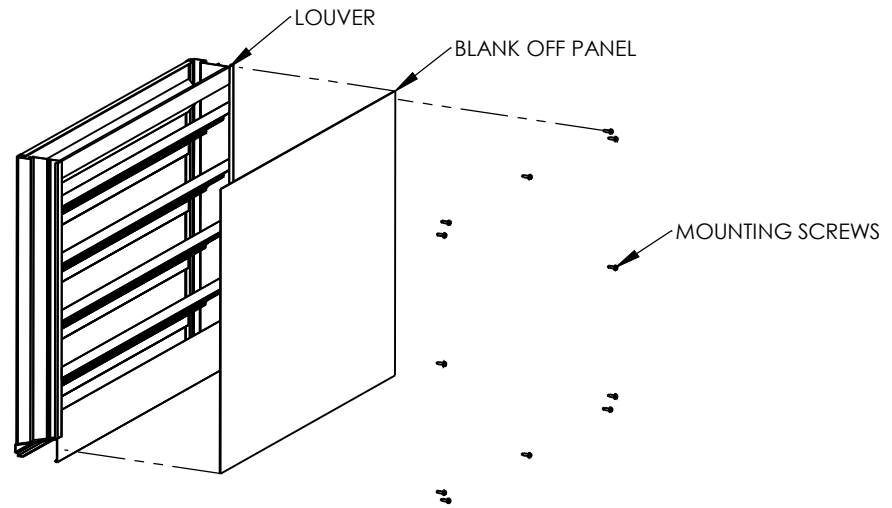
EXPLODED VIEW
