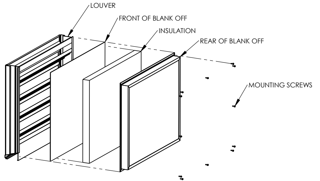
EXPLODED VIEW
