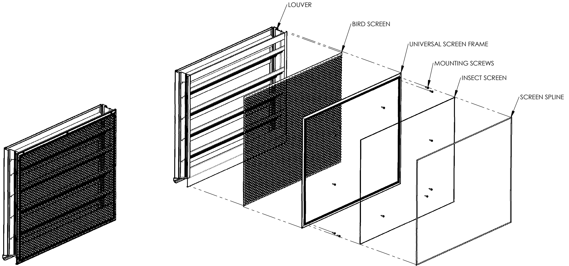
EXPLODED VIEW
