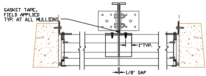
INVISIBLE MULLION W/ANCHOR CLIPS (DOUBLE 1/8" X 5" DEEP CHANNELS SHOWN)
