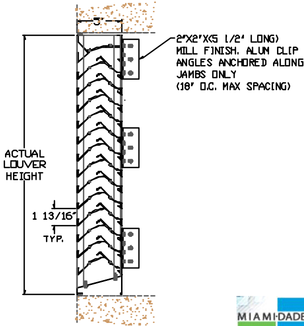
VERTICAL (SINGLE) SECTION
