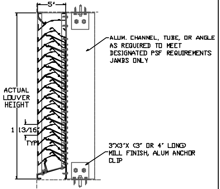
VERTICAL (MULTIPLE) SECTION
