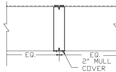
VISIBLE MULLION DETAIL
