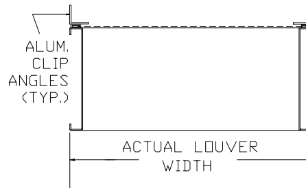
HORIZONTAL SECTION
