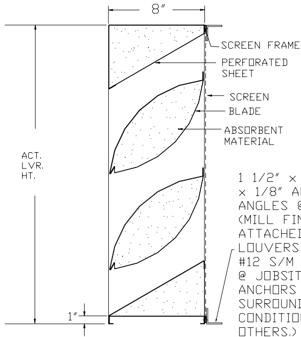
VERTICAL SECTION
