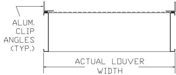
HORIZONTAL SECTION
