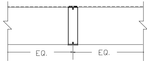
VISIBLE MULLION DETAIL
