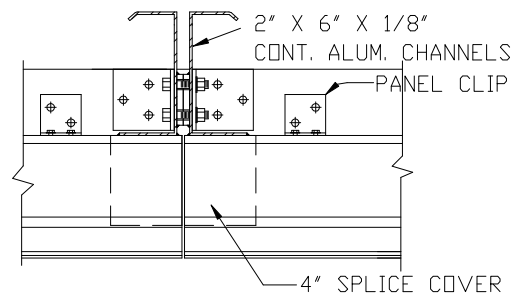
INVISIBLE MULLION DETAIL
