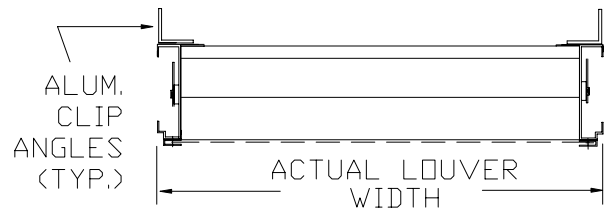
HORIZONTAL SECTION
