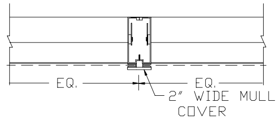
VISIBLE VERTICAL MULLION
