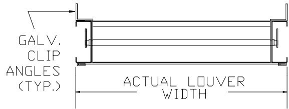
HORIZONTAL SECTION
